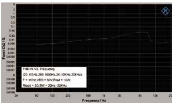
Distortion Spectrum
