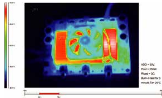
Thermal Image
